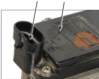
Cracked Plastic Connector and Housing
